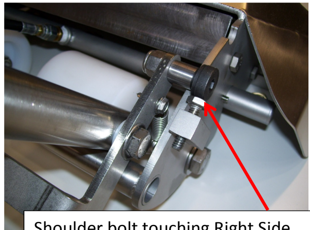
Shoulder bolt touching Right Side Stop Screw
