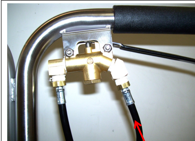
13.75" Solution Hose – NM5691
