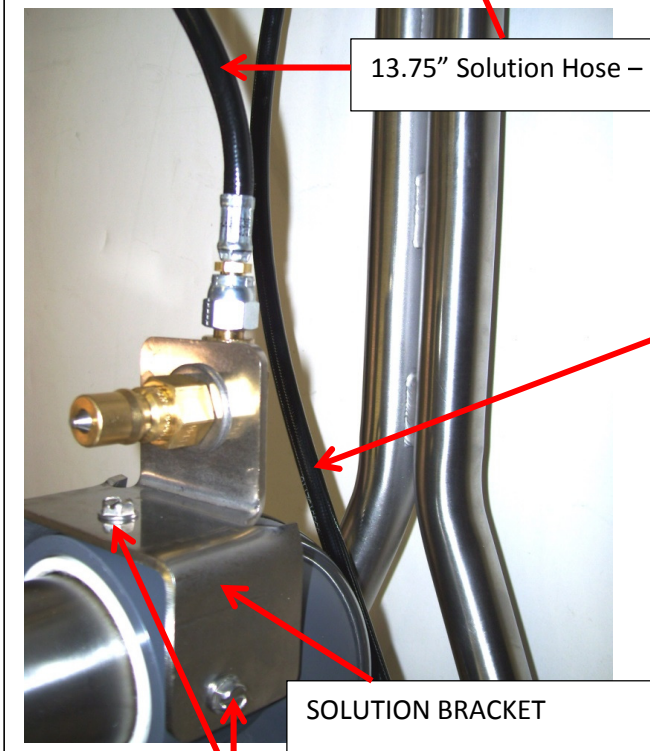
Screw Tek #12 x 5/8" SS – NM4124
